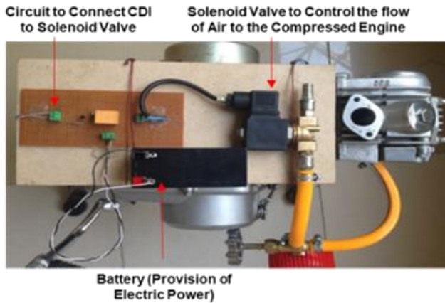
Fig. 7. Electrical circuit for compressed air injection timings
