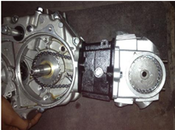
Fig. 3. Crankshaft and camshaft assembly
