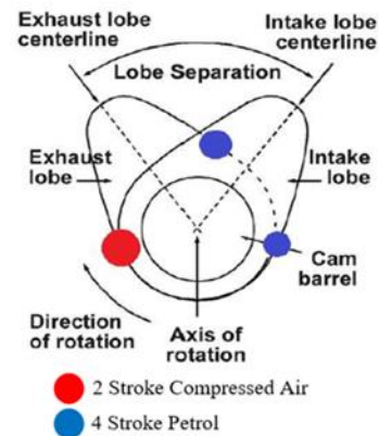
Fig. 5. Position of top dead centre (TDC)
