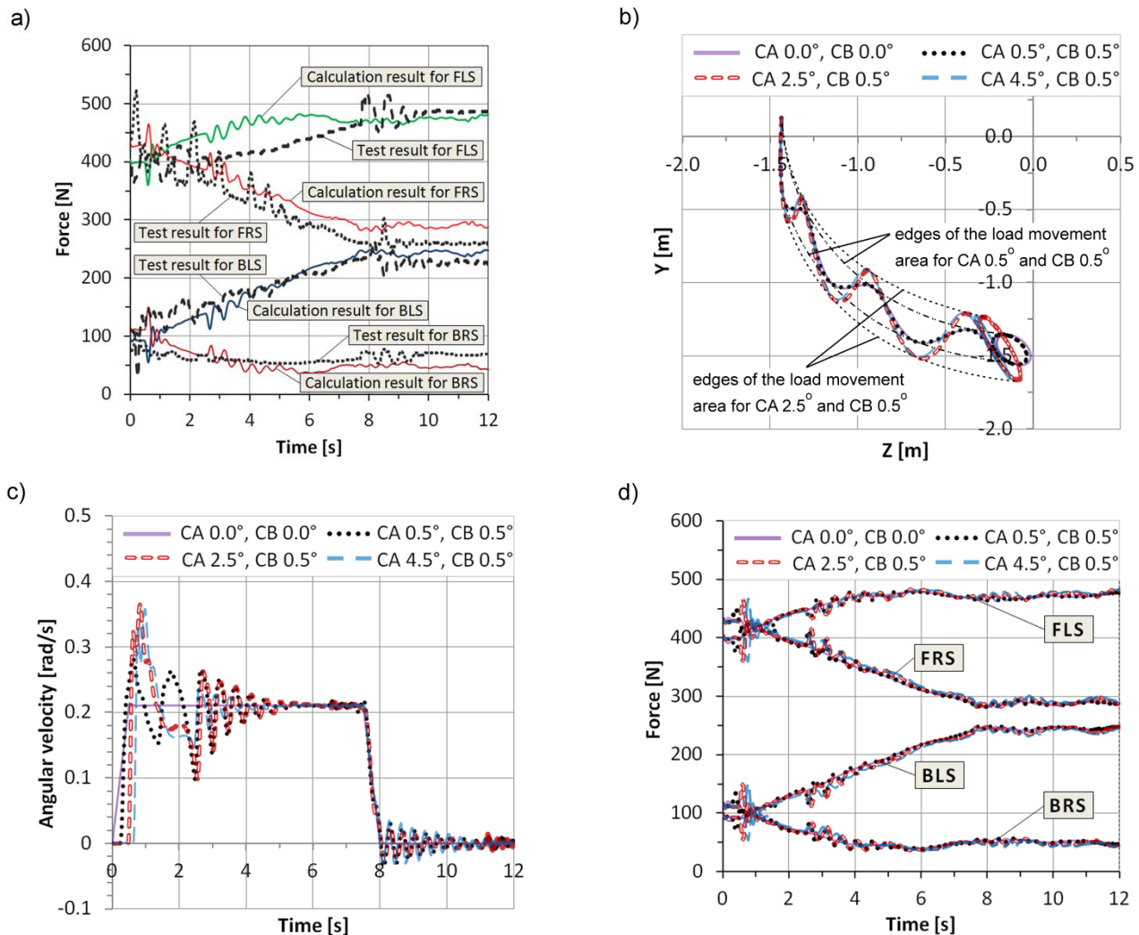
Fig. 6. Calculation results: a) comparison of the support loads - calculated with the one that were recorded during the tests (for 3^\circ clearance), b) trajectory of the mass centre of the load, c) speed of rotation of the body relative to the chassis, d) distribution of the support loads (FLS – front left support, FRS – front right support, BLS – back left support, BRS – back right support)
