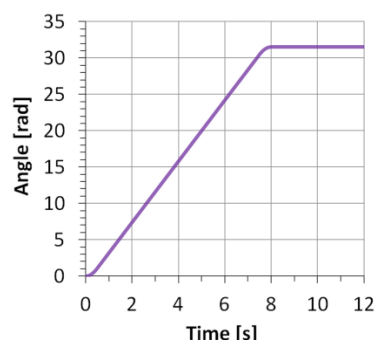
Fig. 4. Slewing motion input function
