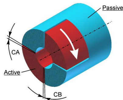
Fig. 5. Clearance model
