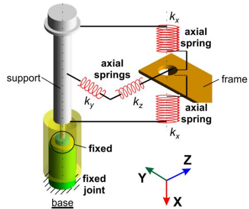
Fig. 2. Support model (Trąbka, 2014b)
