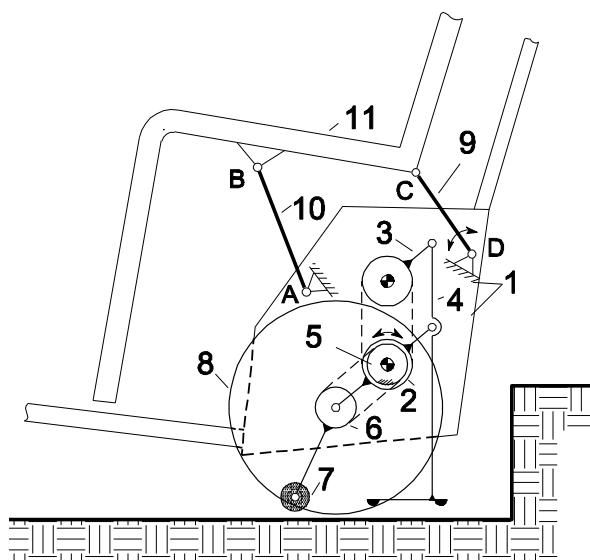
Fig. 4. Kinematic scheme of stair climber with mechanism changing passenger's gravity centre position: 1 – frame, 2 – driving chain wheel, 3 – parallel chain wheel, 4 – foot (parallel chain connecting link), 5 – stationary chain wheel, 6 – satellite chain wheel, 7 – braking wheel, 8 – driving-walking wheels 9 – control mechanism crank, 10 – control mechanism rocker, 11 – seat
