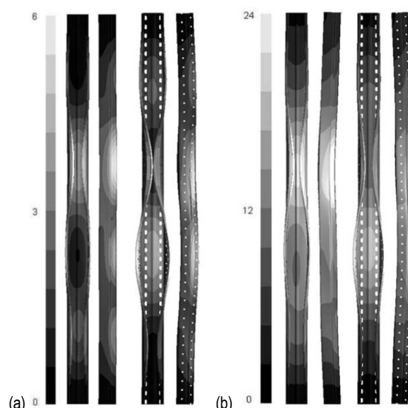
Fig. 11. Section RS125×3.2, brut and net, with the length of 2200 mm: (a) initial shapes for worst imperfection amplified by factor 5.0, (b) deformed shapes at limit load for worst imperfection amplified factor 2.5
