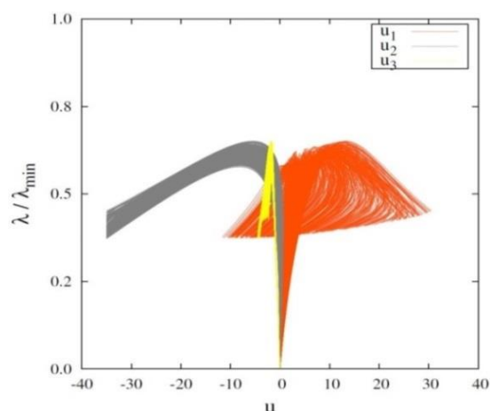
Fig. 10b. Net section RS125×3.2 with length of 2200 mm: equilibrium paths \lambda versus u . The displacement components u_1 , u_2 and u_3 are measured in the point of the middle of the upright pallet rack section
