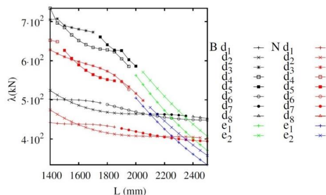
Fig. 7. Buckling load vs. corresponding length for the R125 \times 3.2 brut (B) and net (N) sections
