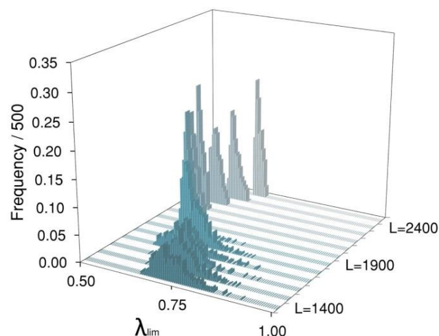
Fig. 12a. Frequency distribution of the limit load found \lambda_{lim} for the RS125×3.2 brut section
