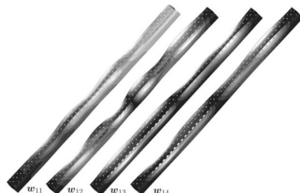
Fig. 9b. Quadratic corrections for the brut section with length of 2200 mm
