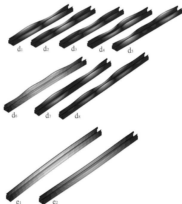
Fig. 6. Distortional d_1, d_2 \dots d_8 and global e_1, e_2 buckling modes for RSN125 \times 3.2 net section in the range L = 1400 \dots 2500 mm
