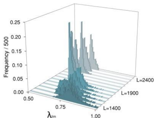
Fig. 12b. Frequency distribution of the limit load found \lambda_{lim} for the RS125×3.2 net section
