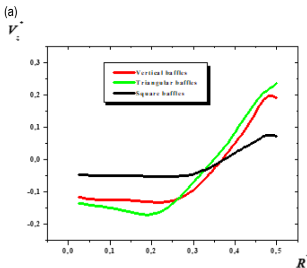
Fig. 11. Axial velocities for different configurations (VBR, TBR and SBR) for Z^* = 0.25 , (a) Re = 8 \times 10^4 , (b) Re = 10^5
