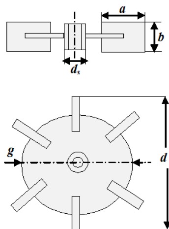
Fig. 1. Geometry of the agitated tank
