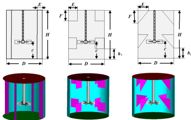
Fig. 1. Geometry of the agitated tank
